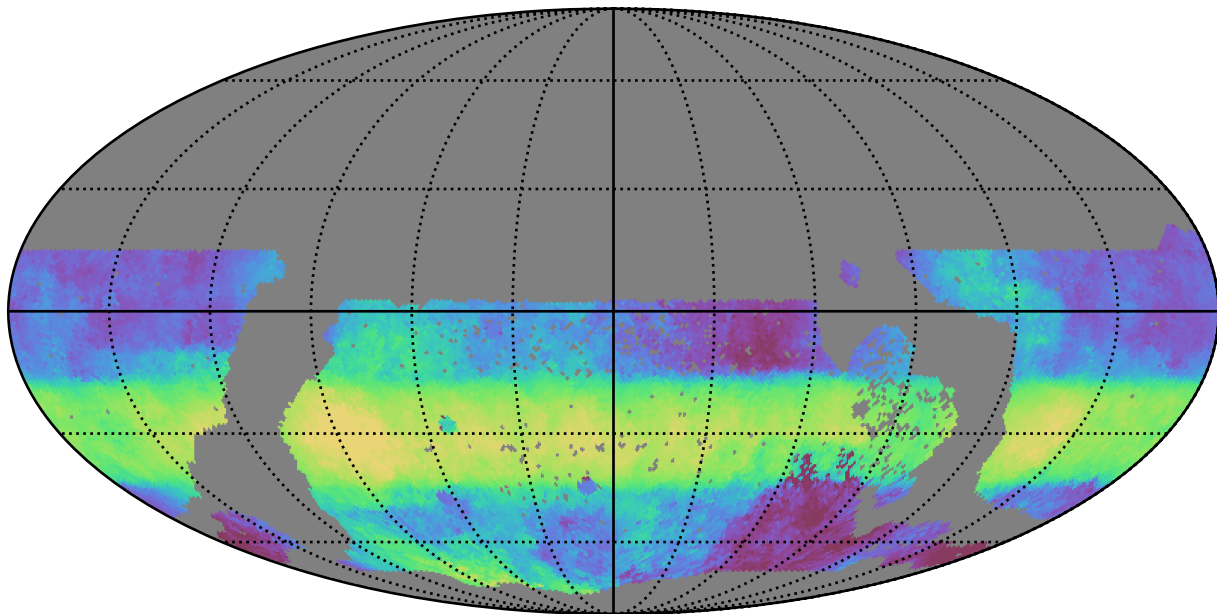
extra_ss_neo7_v3.4_10yrs WFD r band: Median HA
