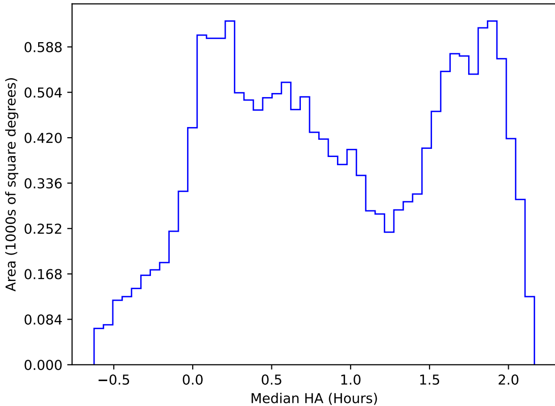
extra_ss_neo7_v3.4_10yrs WFD r band: Median HA
