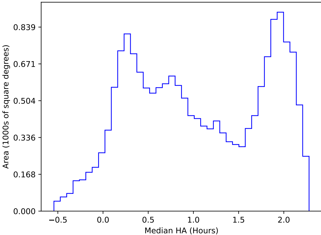
extra_ss_neo7_v3.4_10yrs WFD i band: Median HA
