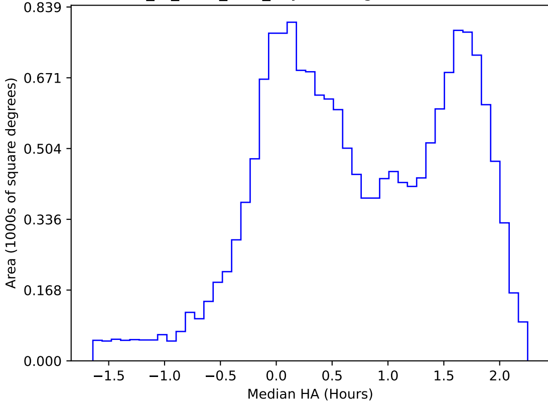
extra_ss_neo7_v3.4_10yrs WFD g band: Median HA
