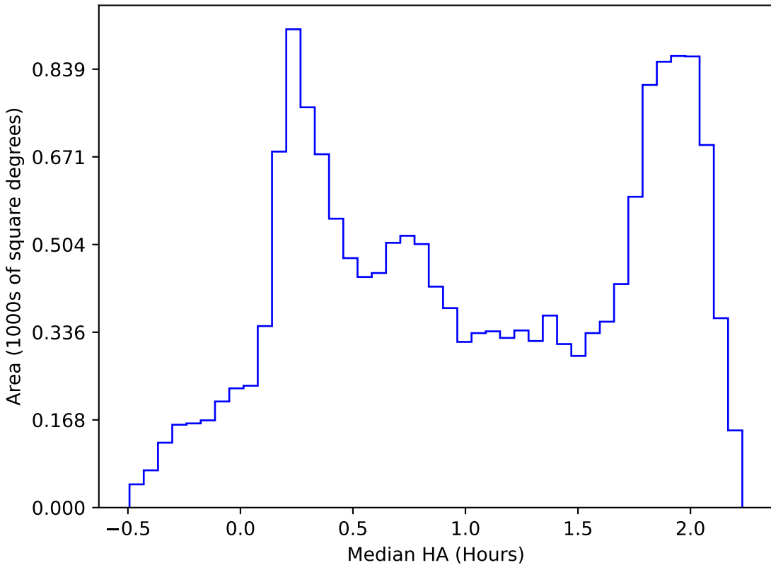
extra_ss_neo7_v3.4_10yrs WFD all bands: Median HA
