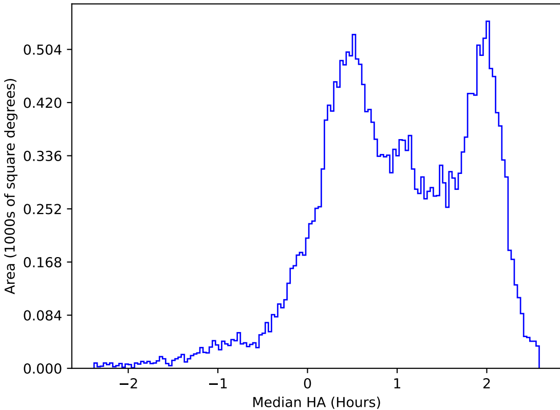
extra_ss_neo7_v3.4_10yrs All sky z band: Median HA
