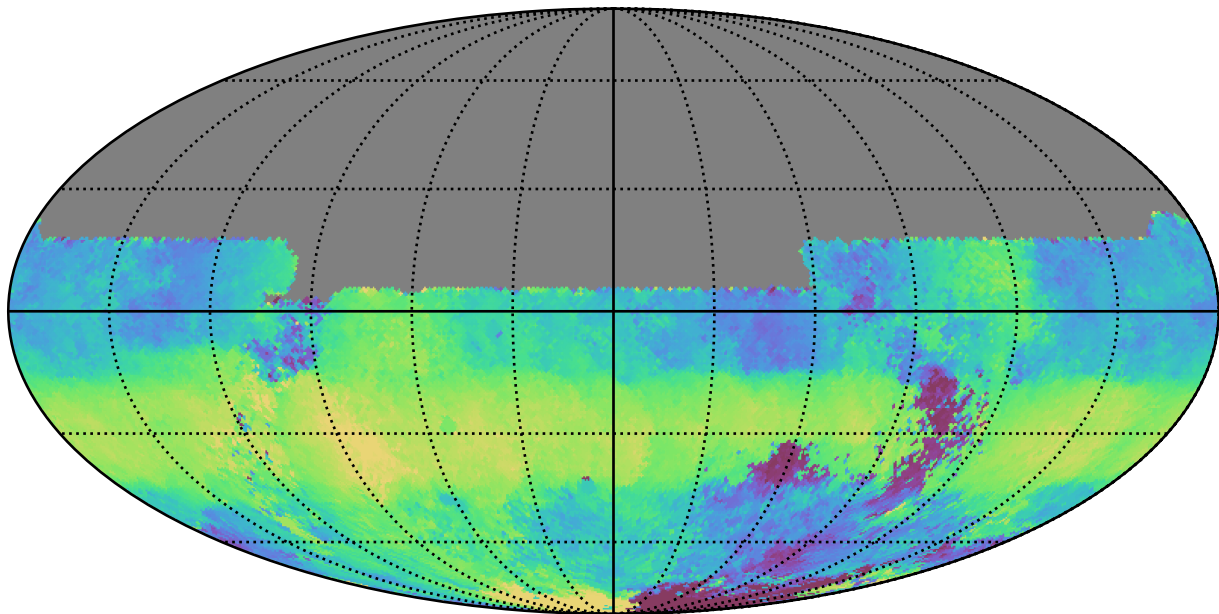
extra_ss_neo7_v3.4_10yrs All sky u band: Median HA
