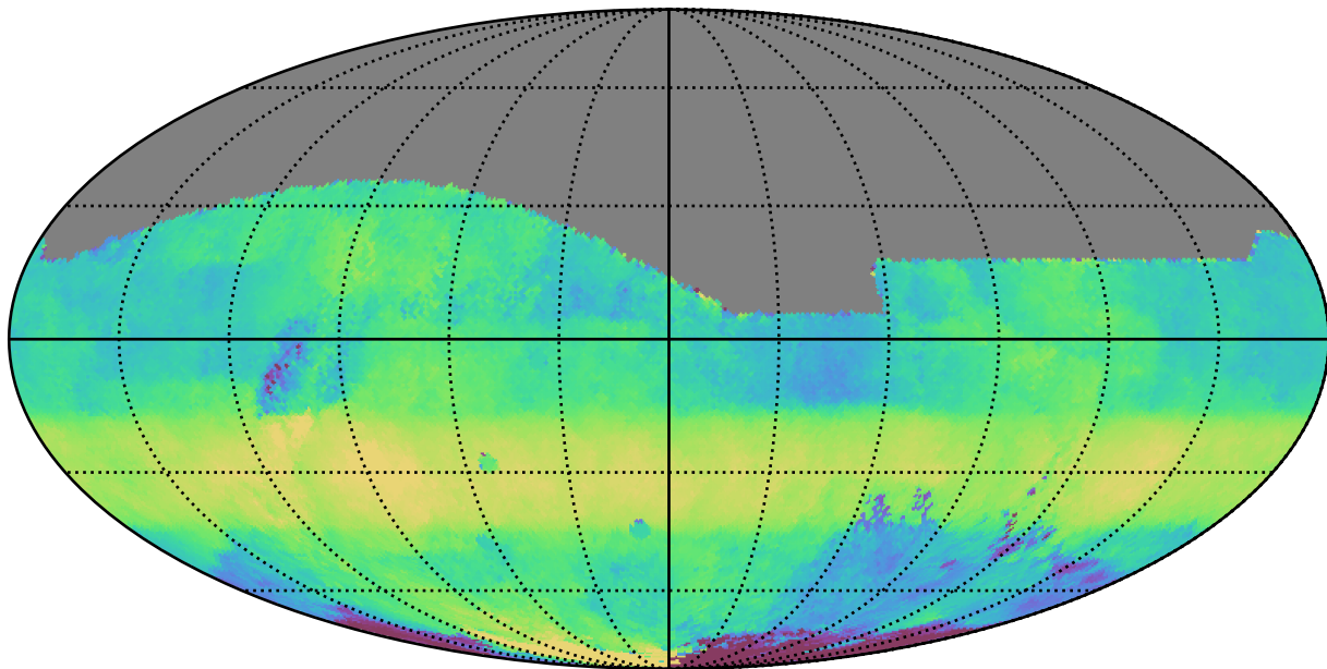
extra_ss_neo7_v3.4_10yrs All sky r band: Median HA
