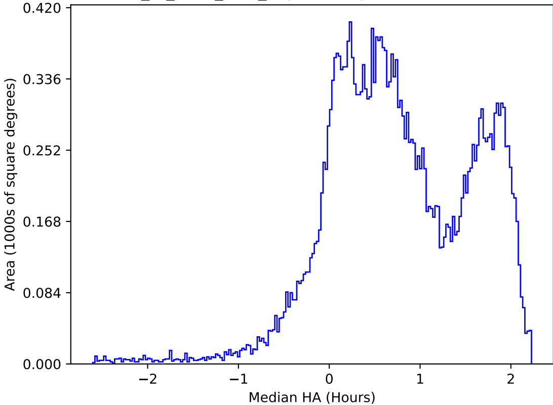
extra_ss_neo7_v3.4_10yrs All sky r band: Median HA
