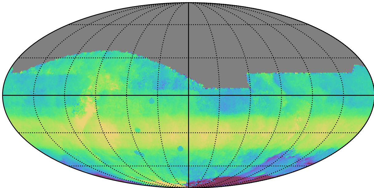
extra_ss_neo7_v3.4_10yrs All sky i band: Median HA
