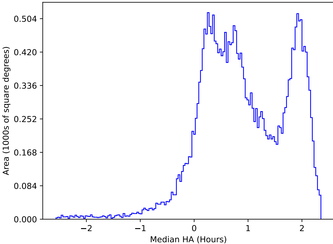
extra_ss_neo7_v3.4_10yrs All sky i band: Median HA
