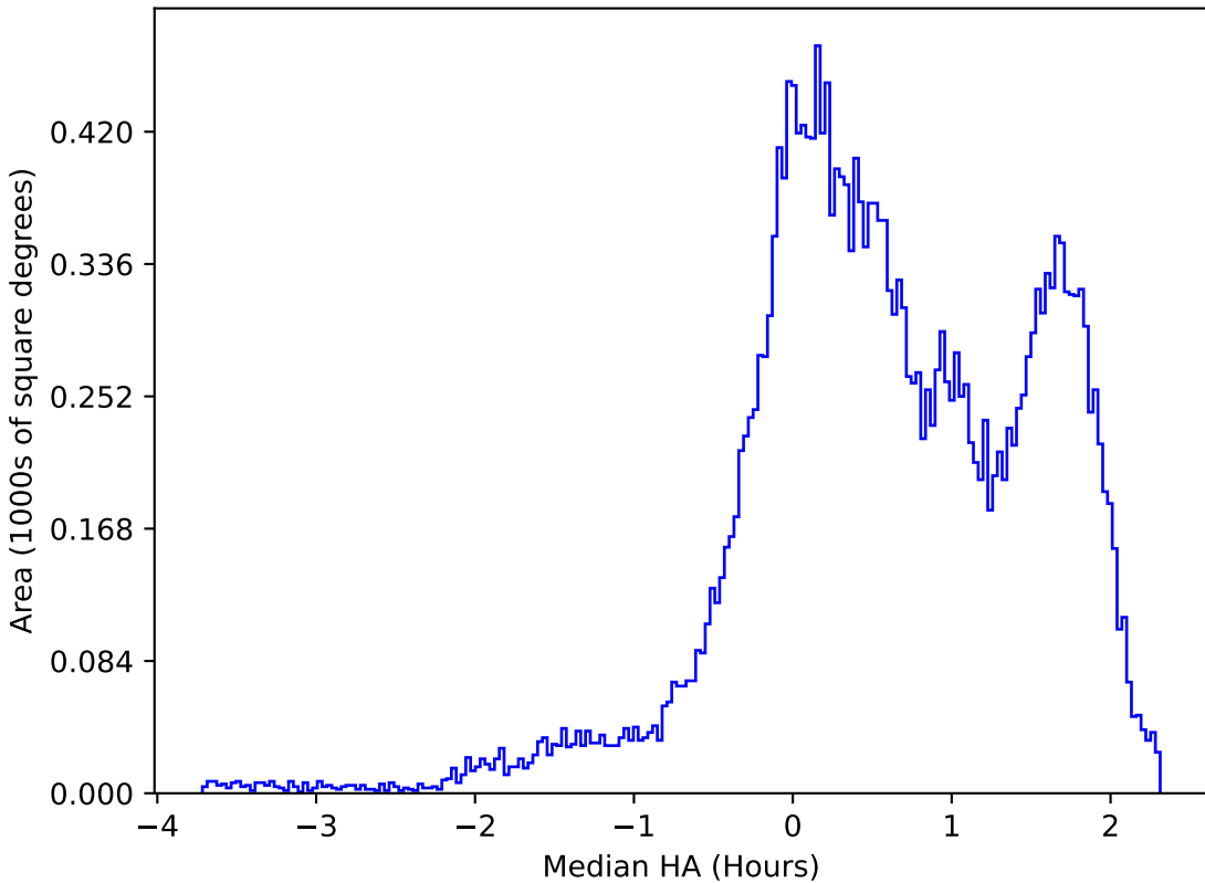
extra_ss_neo7_v3.4_10yrs All sky g band: Median HA
