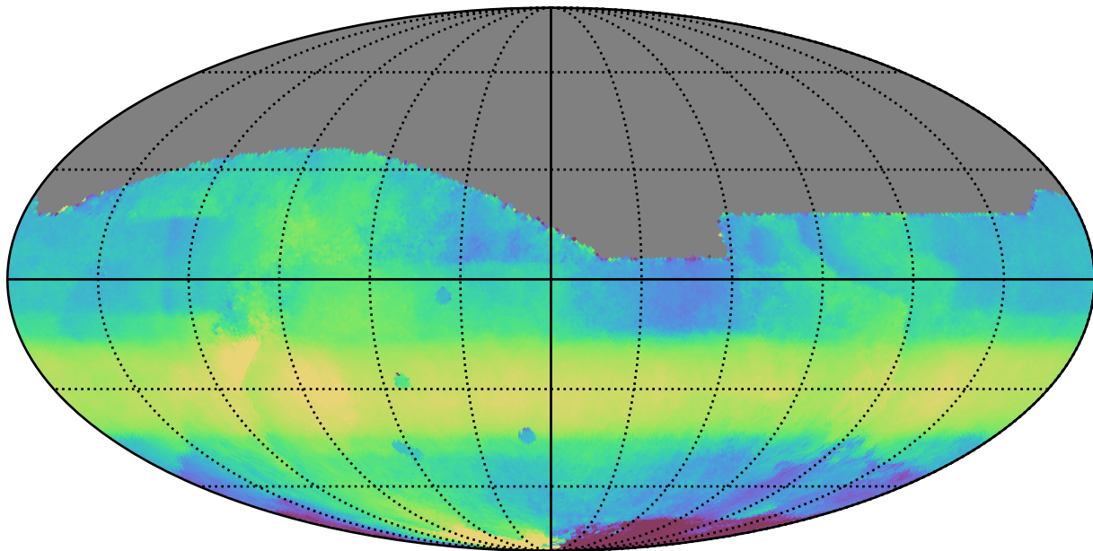
extra_ss_neo7_v3.4_10yrs All sky all bands: Median HA
