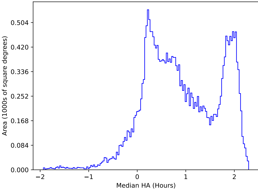
extra_ss_neo7_v3.4_10yrs All sky all bands: Median HA
