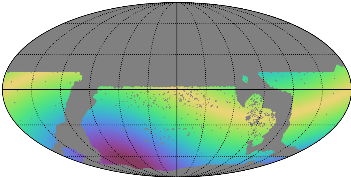
extra_ss_neo7_v3.4_10yrs WFD all bands: Max solarElong
