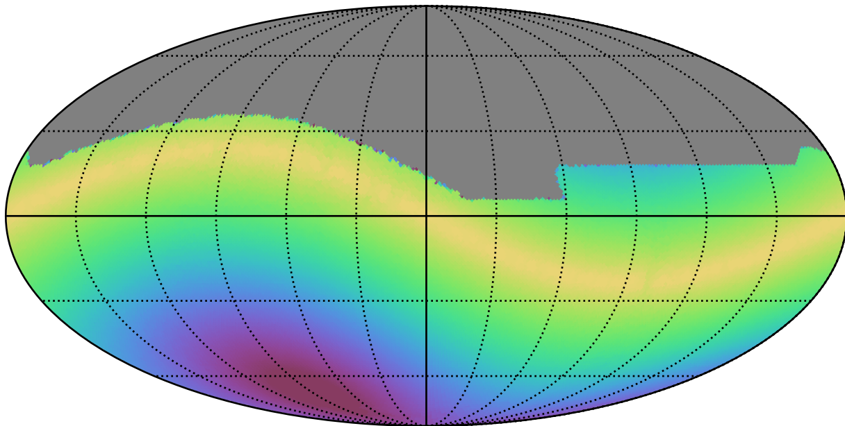
extra_ss_neo7_v3.4_10yrs All sky all bands: Max solarElong
