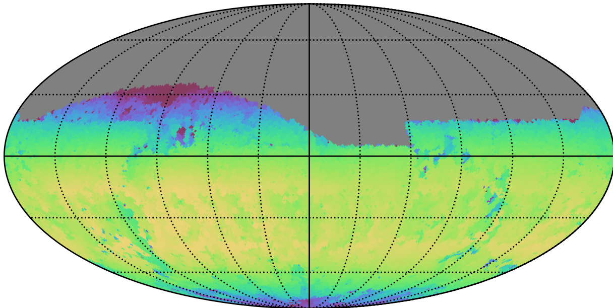
extra_ss_neo7_v3.4_10yrs Yr 1 z band: Max skyBrightness
