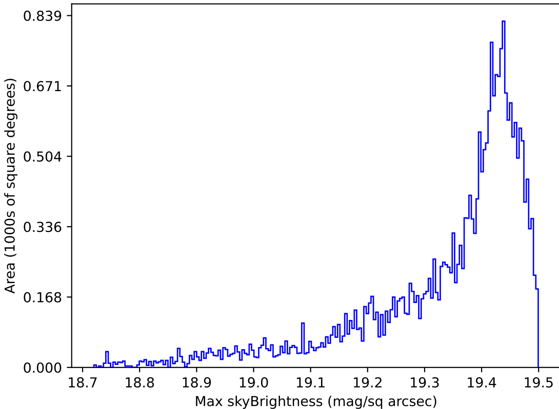
extra_ss_neo7_v3.4_10yrs Yr 1 z band: Max skyBrightness
