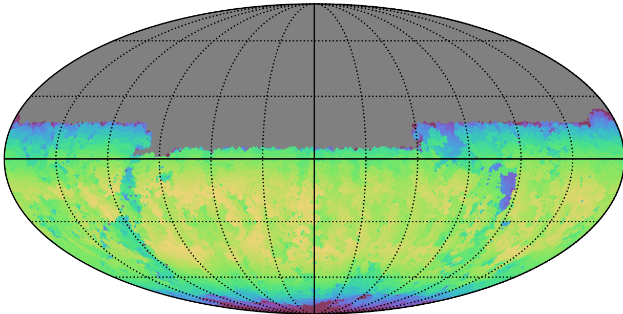
extra_ss_neo7_v3.4_10yrs Yr 1 y band: Max skyBrightness
