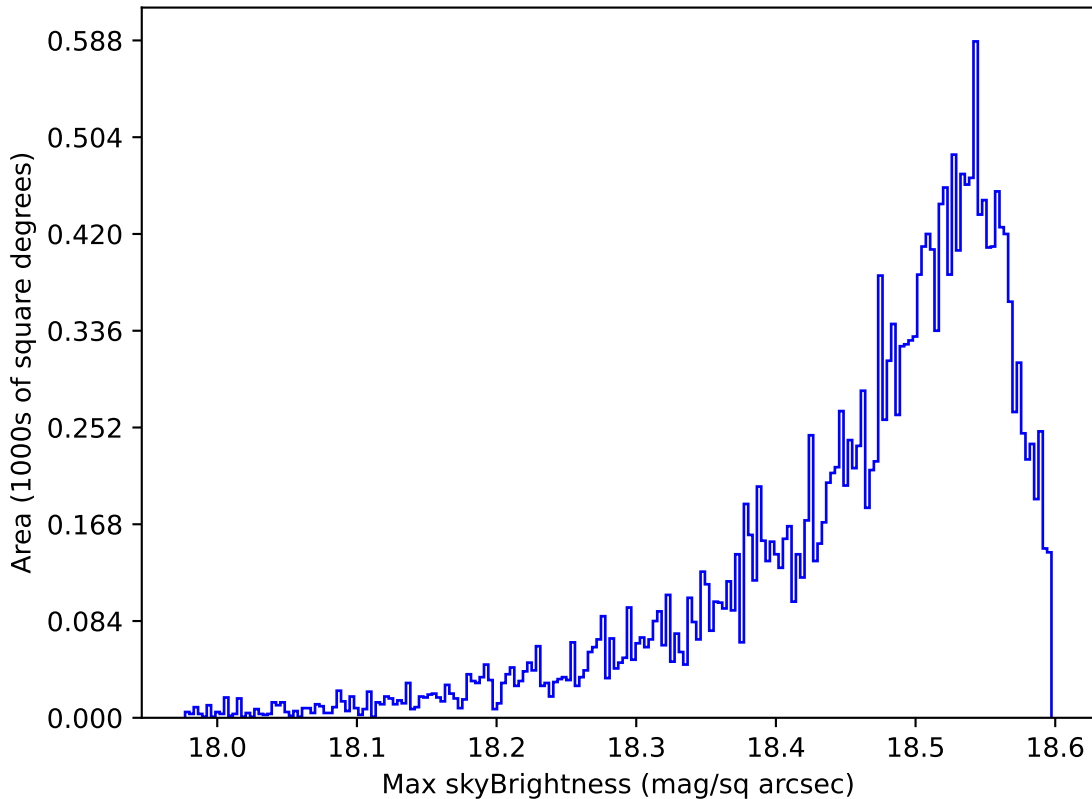
extra_ss_neo7_v3.4_10yrs Yr 1 y band: Max skyBrightness
