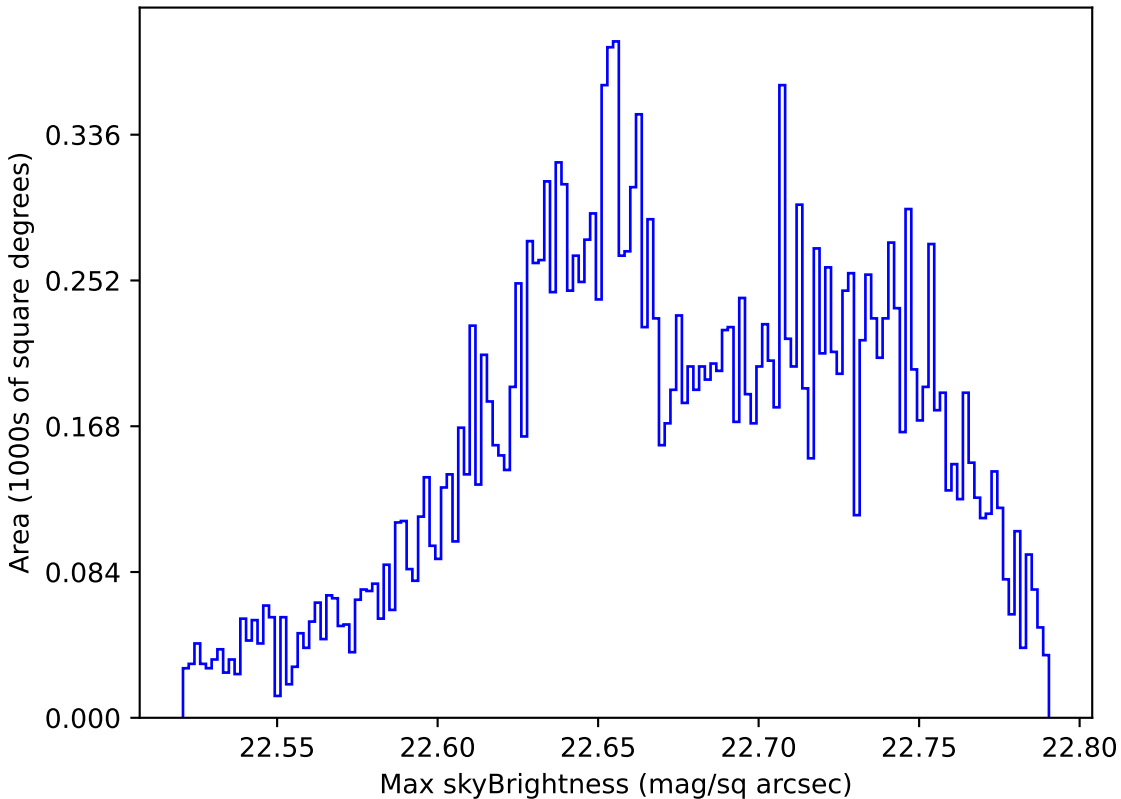
extra_ss_neo7_v3.4_10yrs Yr 1 u band: Max skyBrightness
