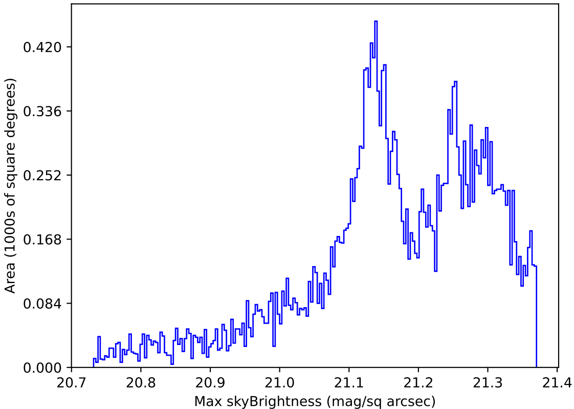
extra_ss_neo7_v3.4_10yrs Yr 1 r band: Max skyBrightness
