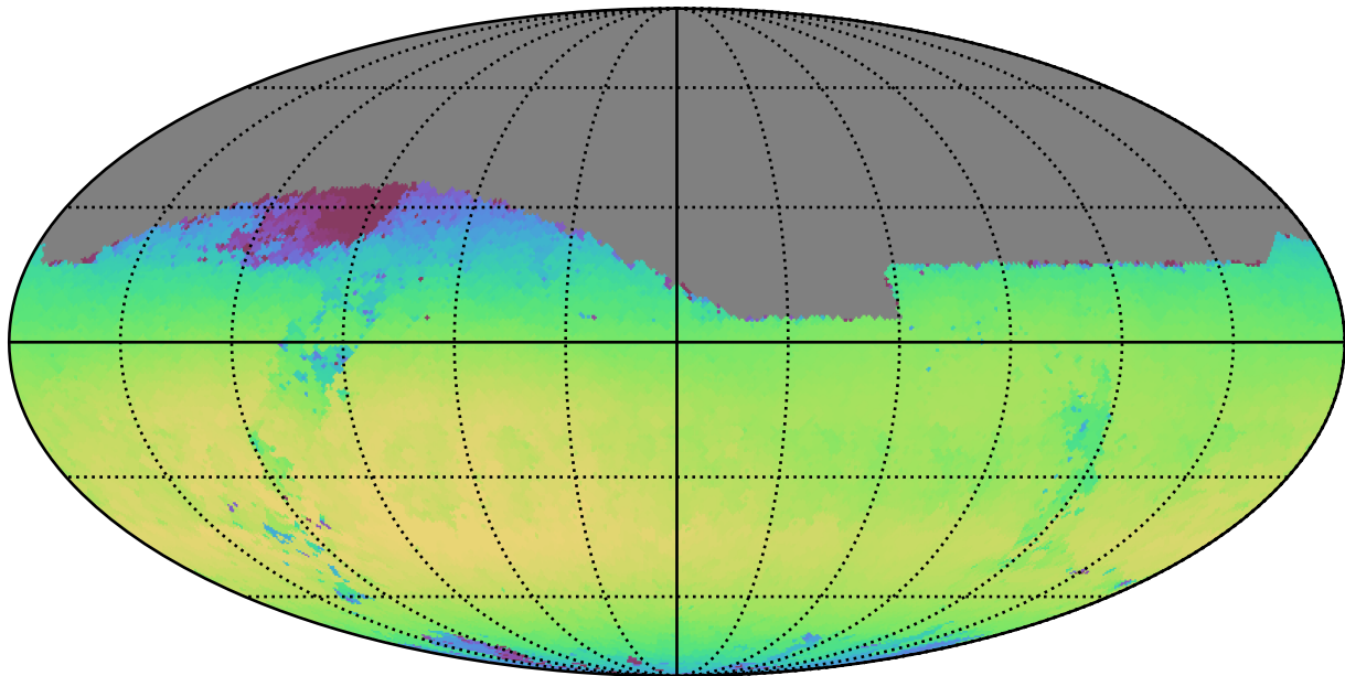
extra_ss_neo7_v3.4_10yrs Yr1 i band: Max skyBrightness
