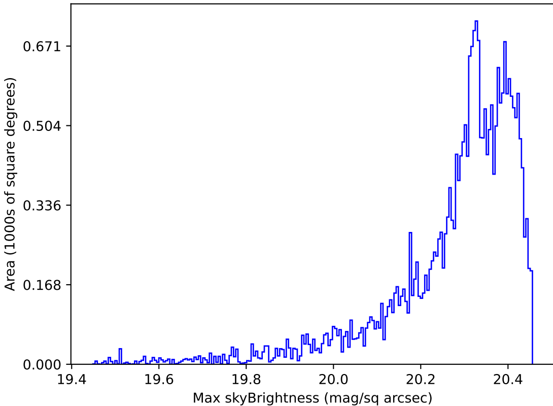
extra_ss_neo7_v3.4_10yrs Yr 1 i band: Max skyBrightness
