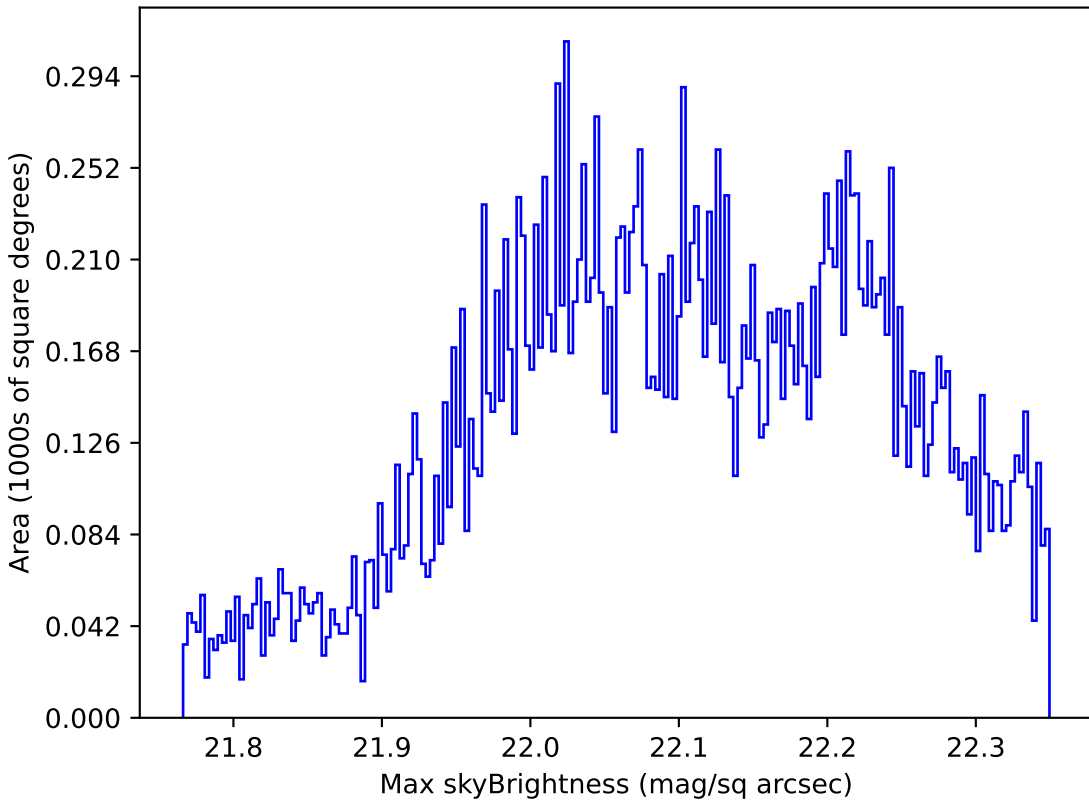
extra_ss_neo7_v3.4_10yrs Yr 1 g band: Max skyBrightness
