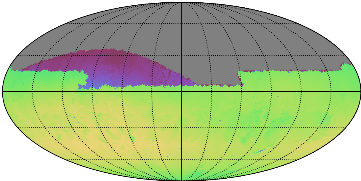
extra_ss_neo7_v3.4_10yrs Yr 1 all bands: Max skyBrightness
