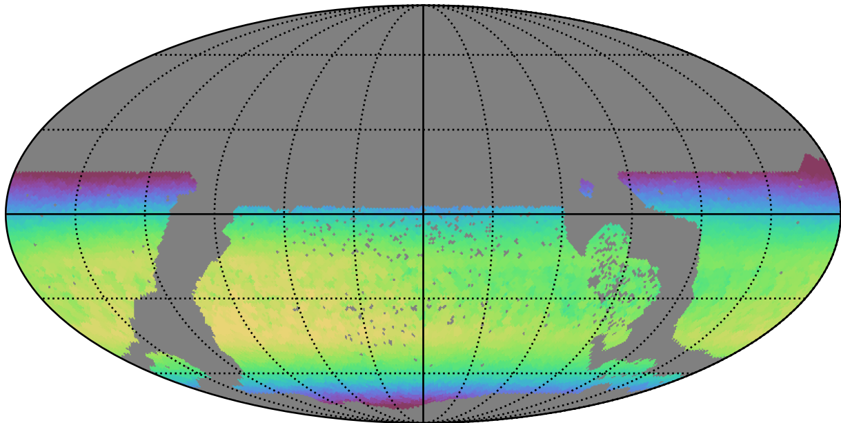
extra_ss_neo7_v3.4_10yrs WFD z band: Max skyBrightness
