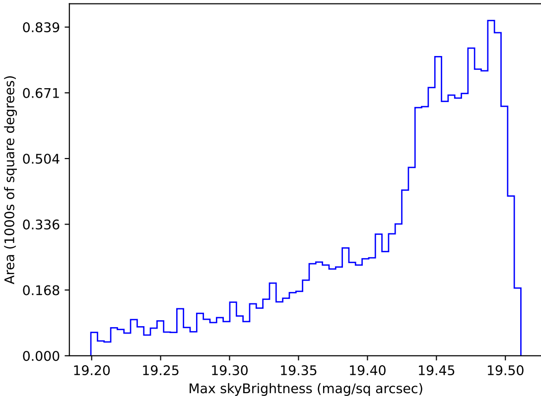
extra_ss_neo7_v3.4_10yrs WFD z band: Max skyBrightness
