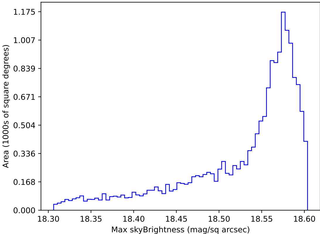
extra_ss_neo7_v3.4_10yrs WFD y band: Max skyBrightness
