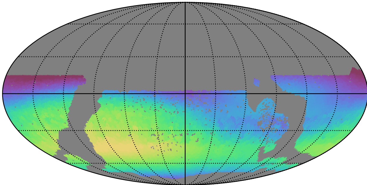
extra_ss_neo7_v3.4_10yrs WFD u band: Max skyBrightness
