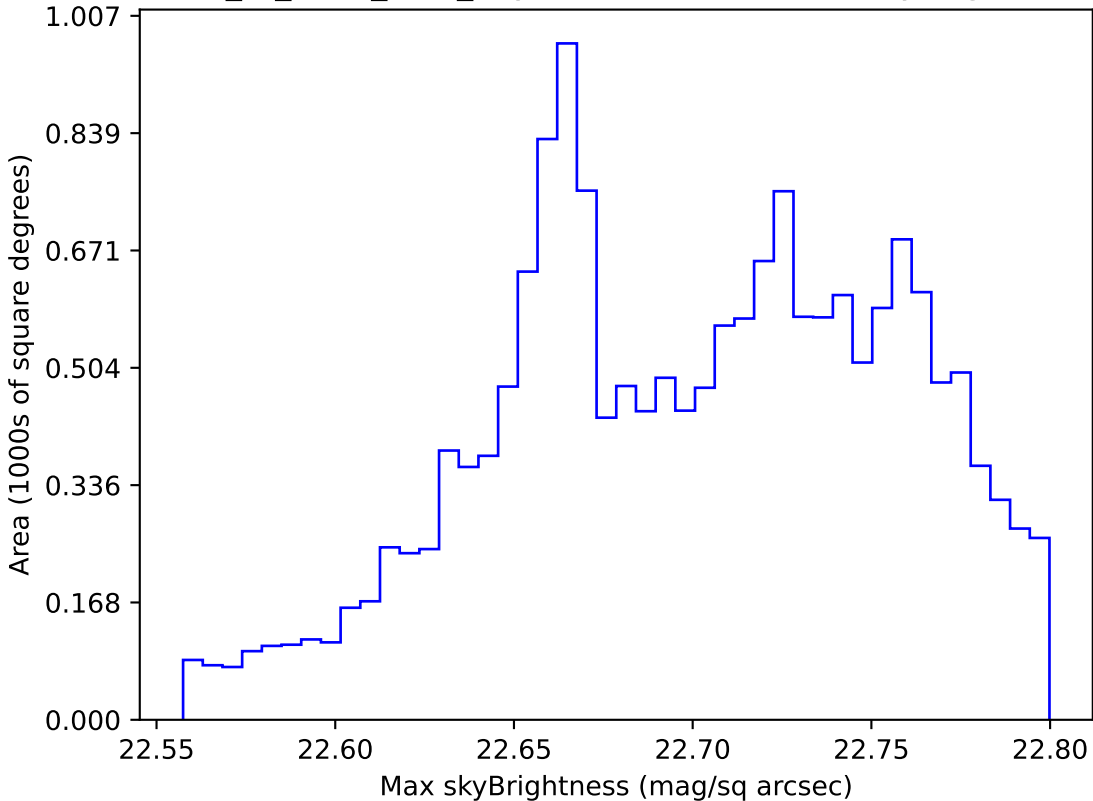
extra_ss_neo7_v3.4_10yrs WFD u band: Max skyBrightness
