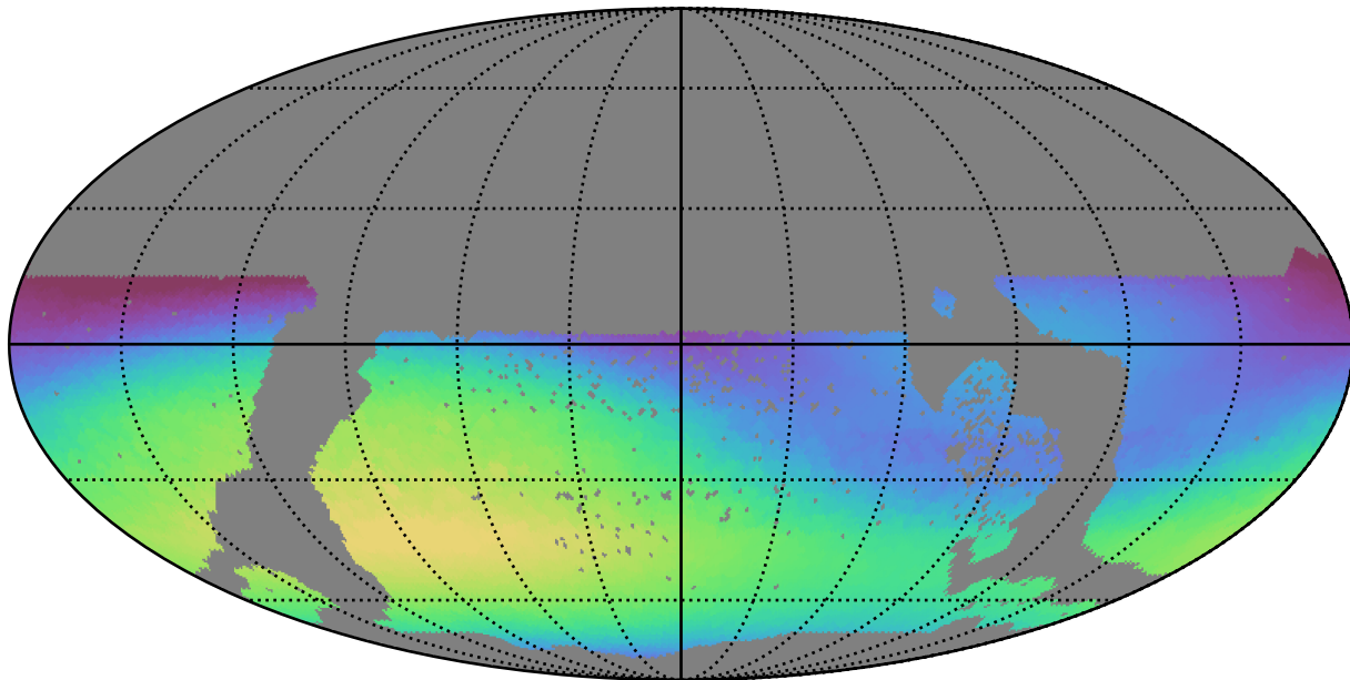
extra_ss_neo7_v3.4_10yrs WFD r band: Max skyBrightness
