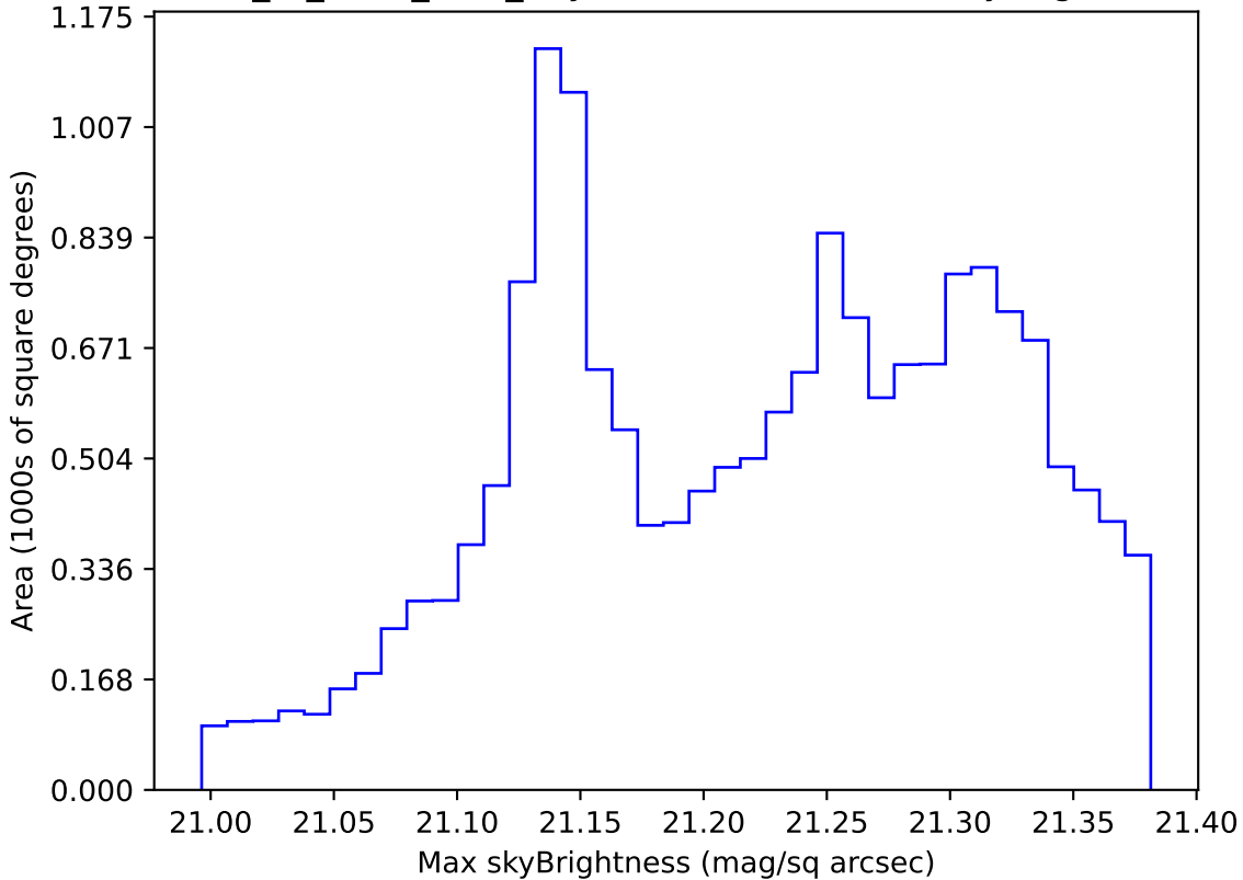
extra_ss_neo7_v3.4_10yrs WFD r band: Max skyBrightness
