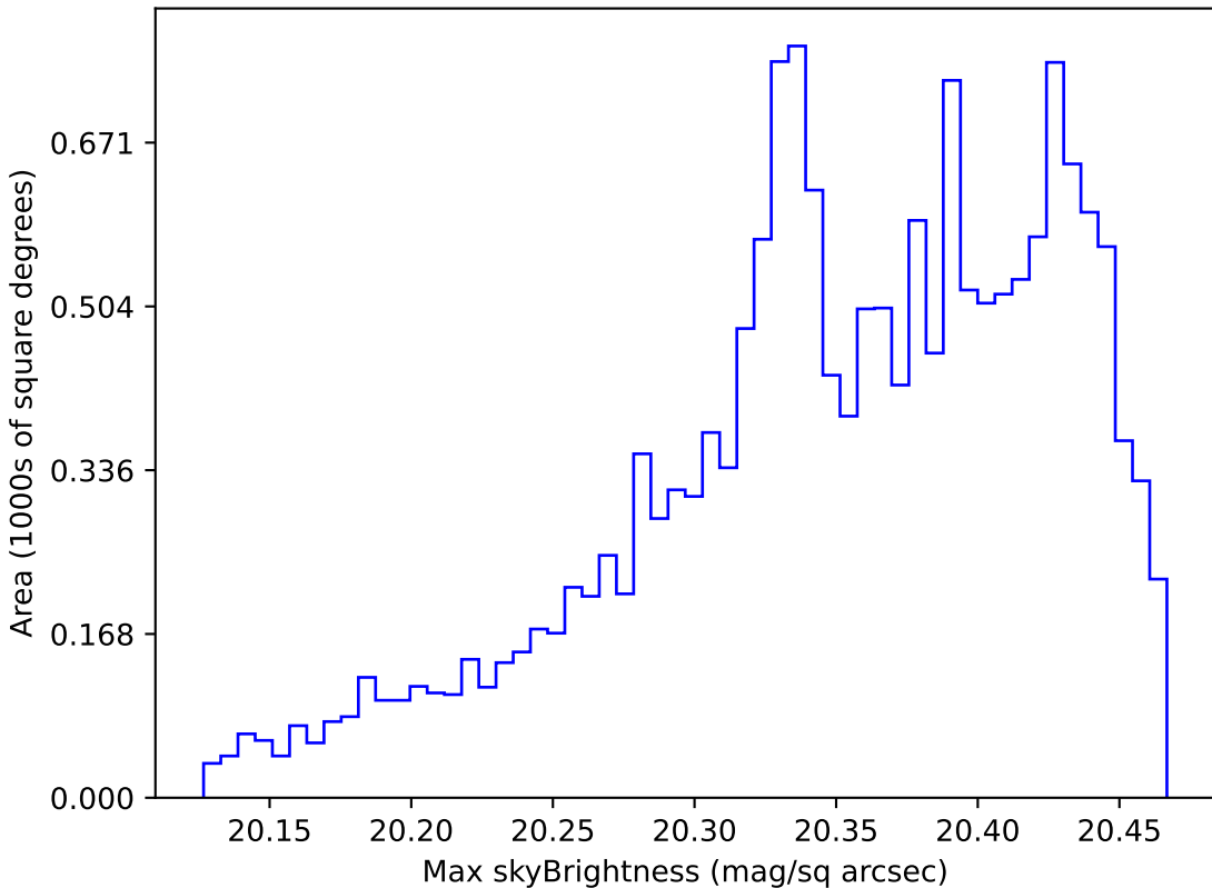
extra_ss_neo7_v3.4_10yrs WFD i band: Max skyBrightness
