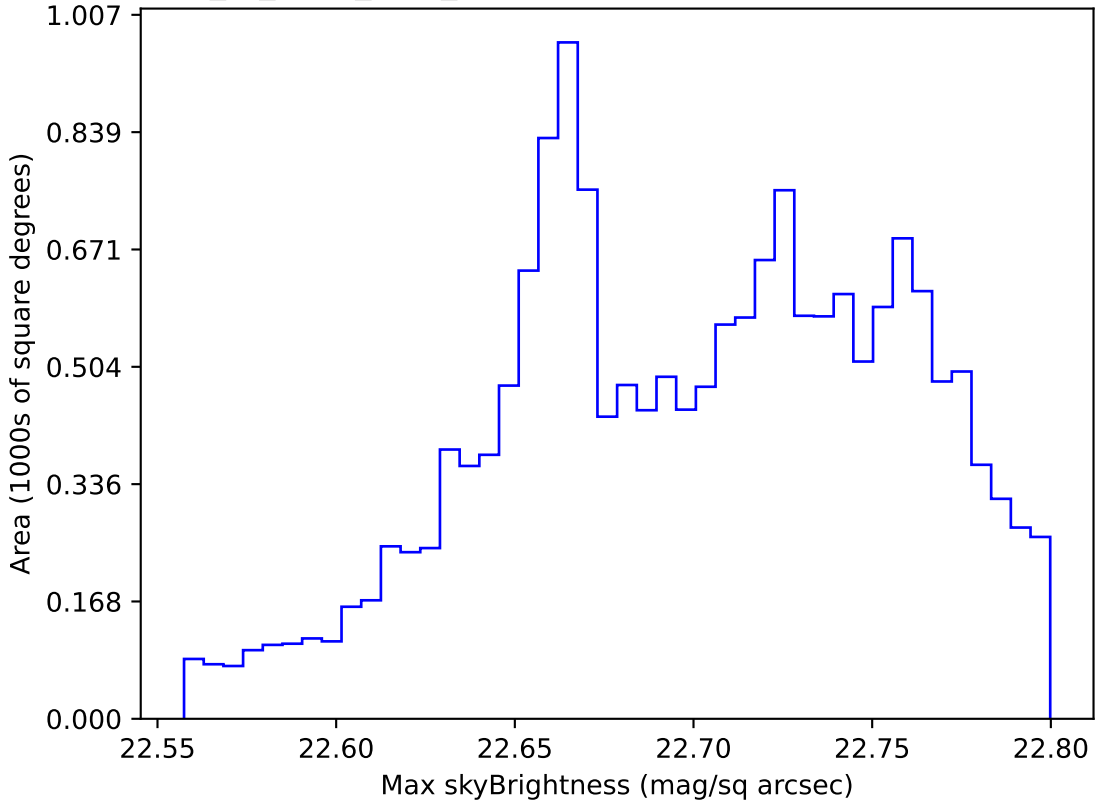
extra_ss_neo7_v3.4_10yrs WFD all bands: Max skyBrightness
