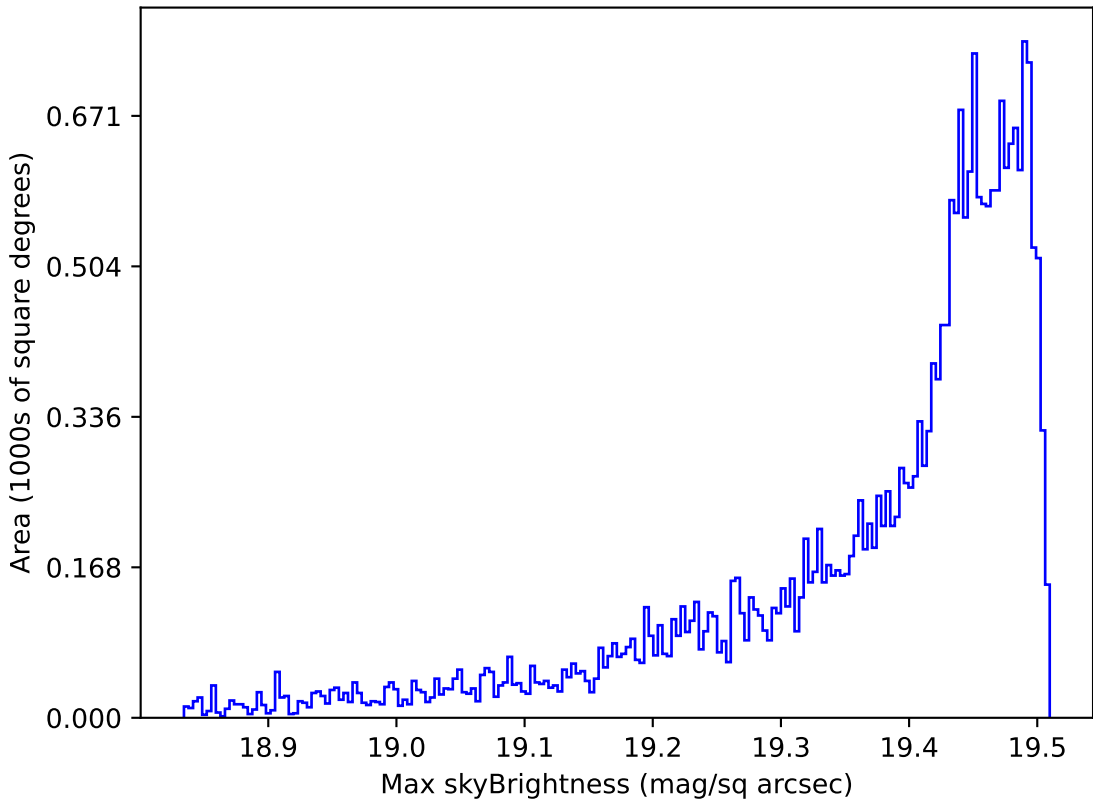
extra_ss_neo7_v3.4_10yrs All sky z band: Max skyBrightness
