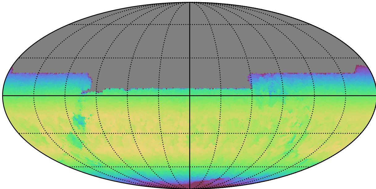
extra_ss_neo7_v3.4_10yrs All sky y band: Max skyBrightness
