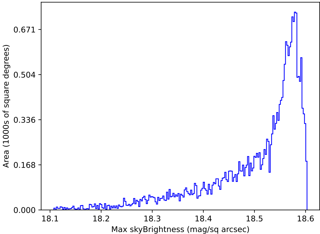
extra_ss_neo7_v3.4_10yrs All sky y band: Max skyBrightness
