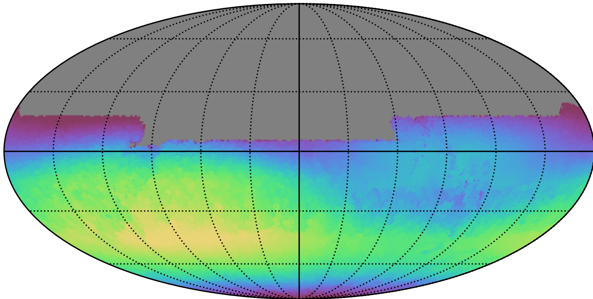
extra_ss_neo7_v3.4_10yrs All sky u band: Max skyBrightness
