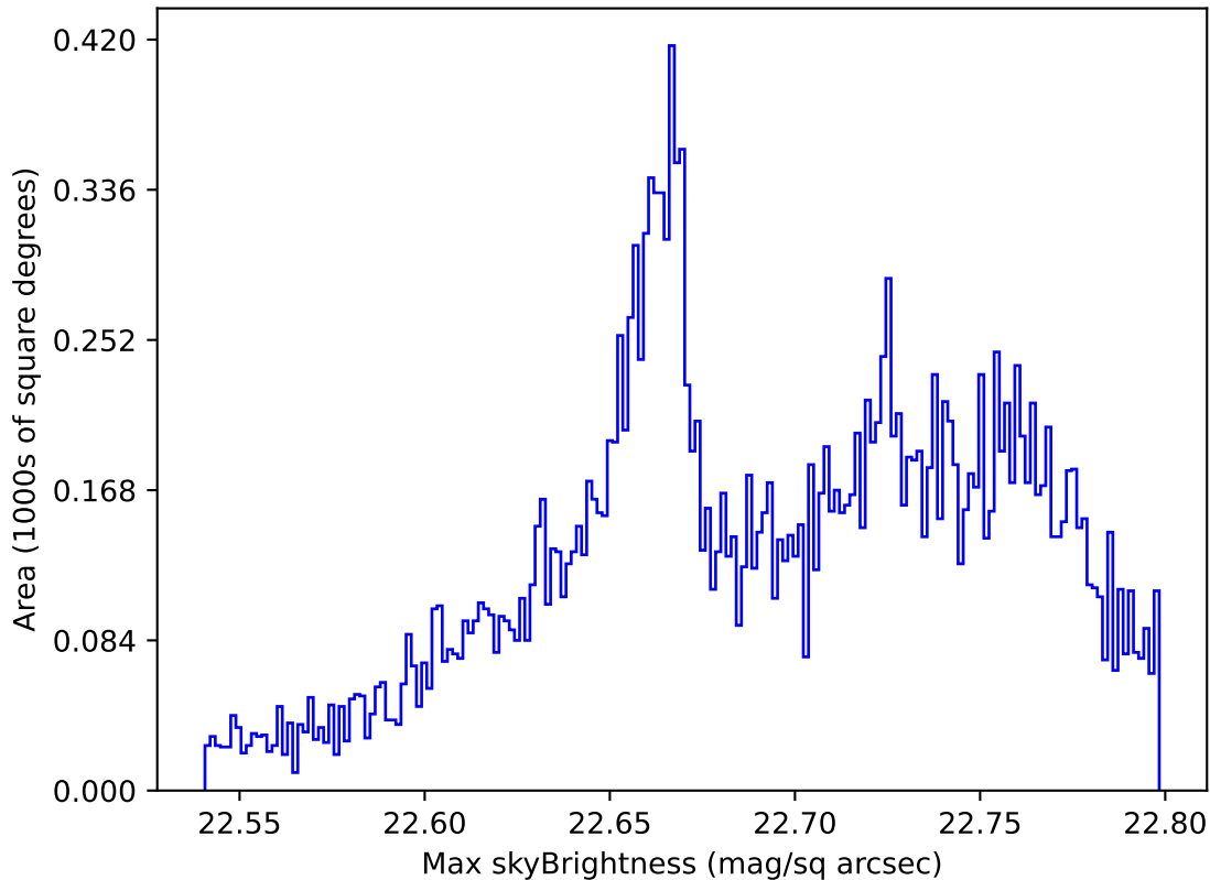
extra_ss_neo7_v3.4_10yrs All sky u band: Max skyBrightness
