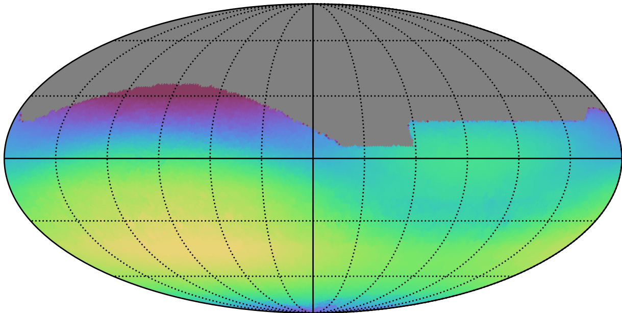
extra_ss_neo7_v3.4_10yrs All sky r band: Max skyBrightness
