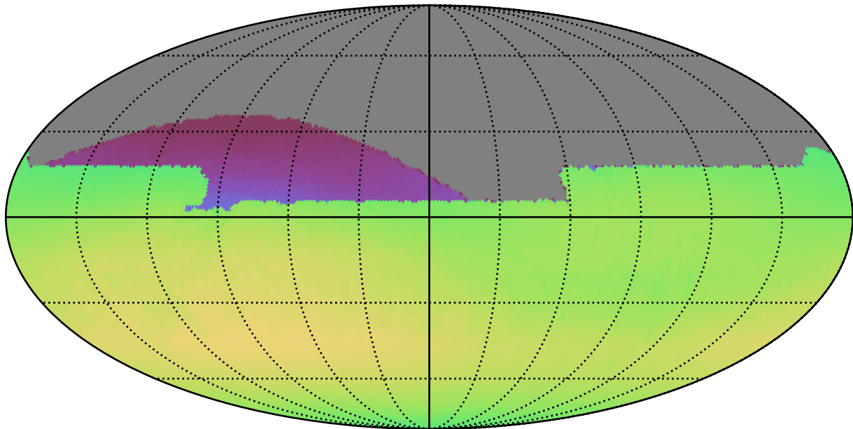
extra_ss_neo7_v3.4_10yrs All sky all bands: Max skyBrightness
