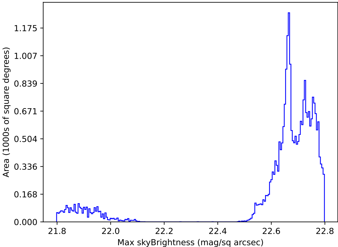
extra_ss_neo7_v3.4_10yrs All sky all bands: Max skyBrightness
