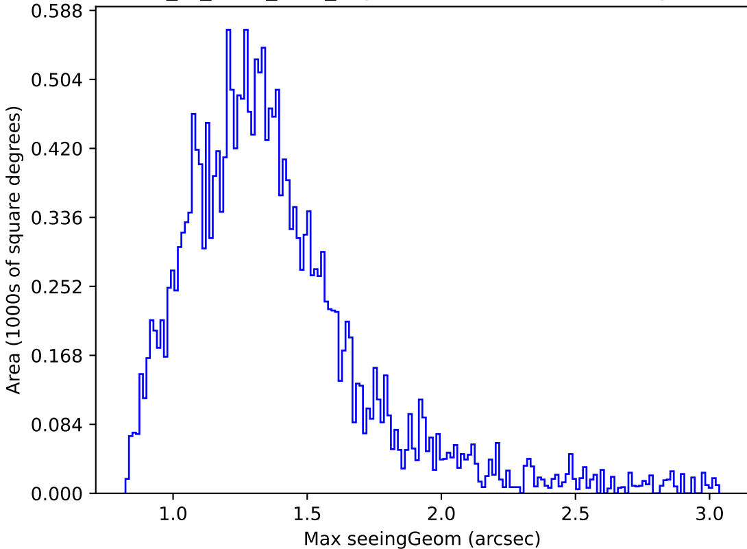
extra_ss_neo7_v3.4_10yrs Yr 1 u band: Max seeingGeom
