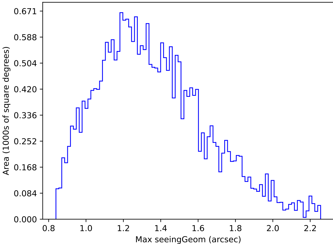
extra_ss_neo7_v3.4_10yrs Yr 1 r band: Max seeingGeom
