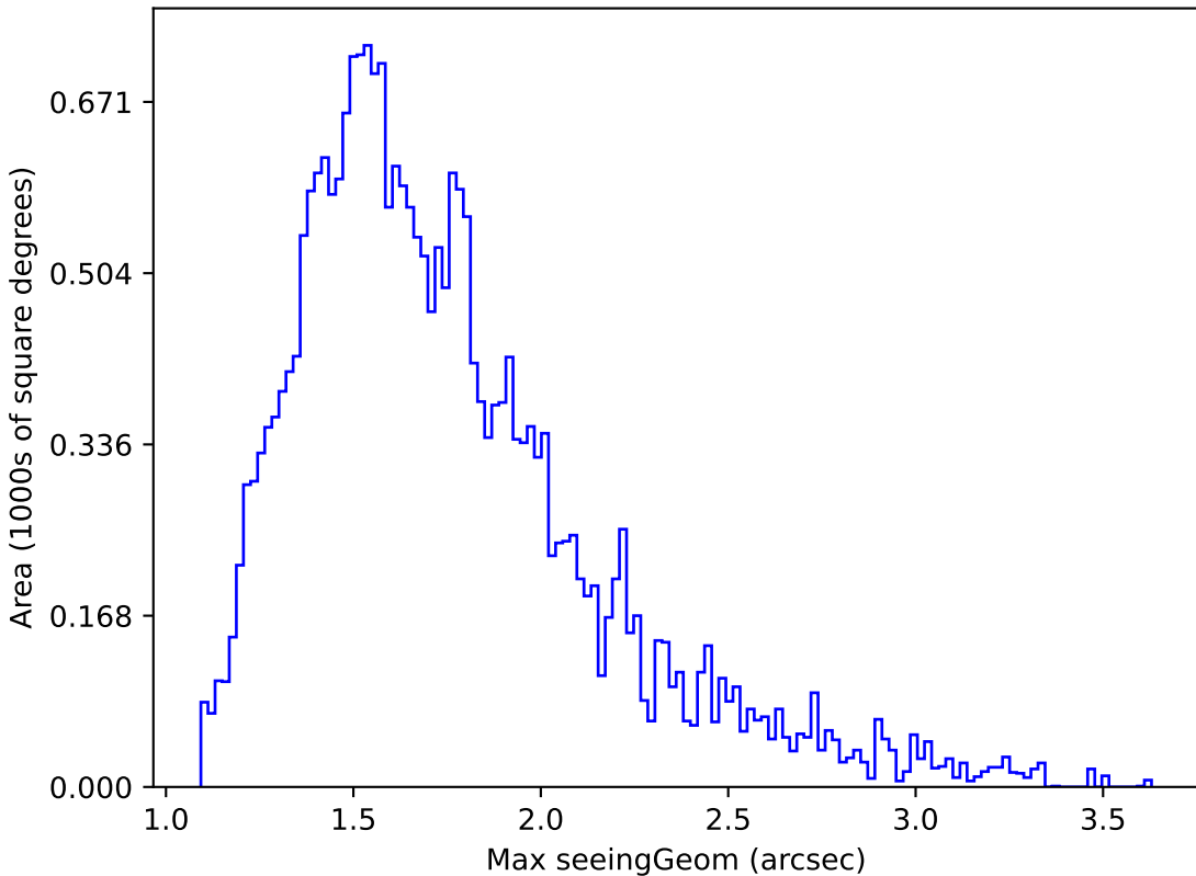
extra_ss_neo7_v3.4_10yrs Yr 1 all bands: Max seeingGeom
