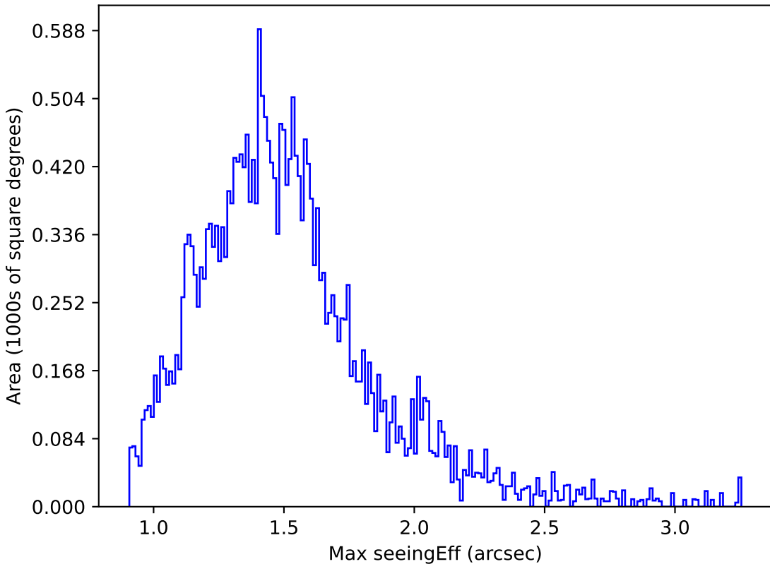
extra_ss_neo7_v3.4_10yrs Yr 1 z band: Max seeingEff
