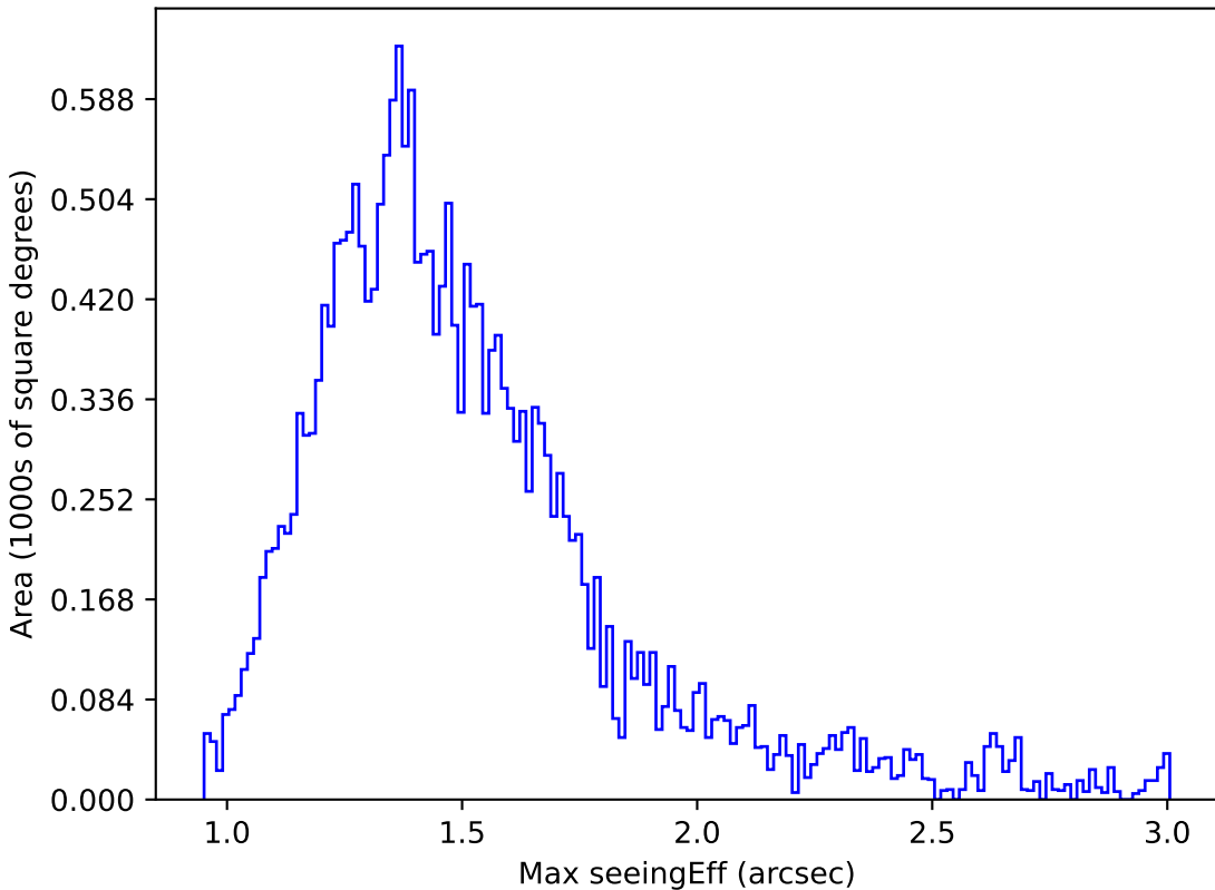
extra_ss_neo7_v3.4_10yrs Yr 1 y band: Max seeingEff
