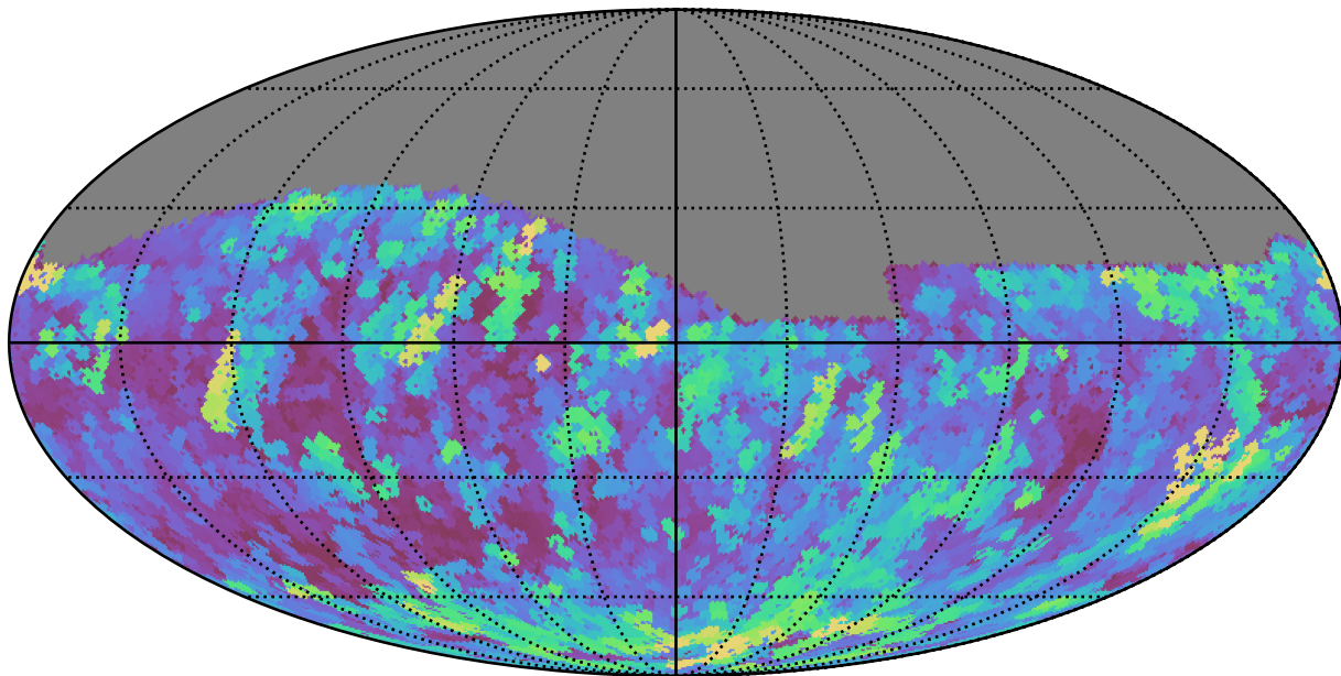
extra_ss_neo7_v3.4_10yrs Yr 1 r band: Max seeingEff
