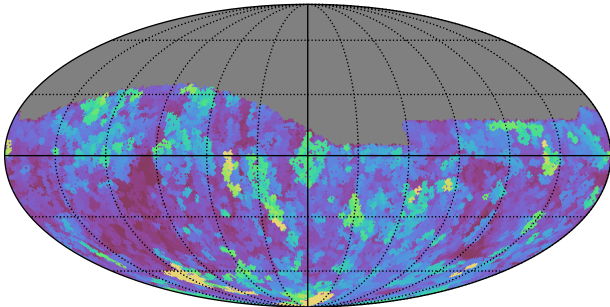
extra_ss_neo7_v3.4_10yrs Yr 1 i band: Max seeingEff
